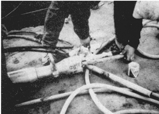
Figure 5-14. Plug-and-feather splitter
